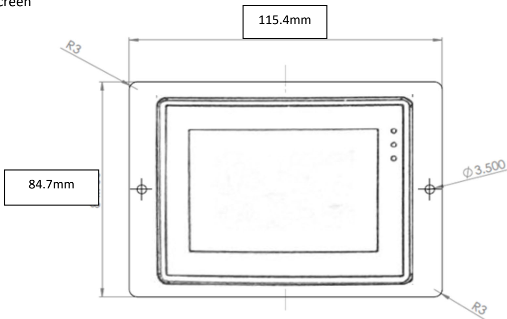
Fig. 25 Touch screen dimensions
