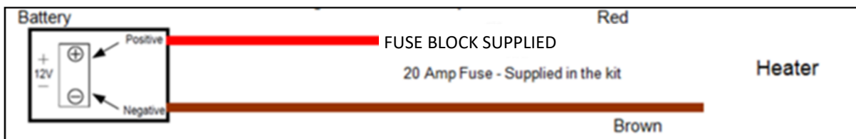
Fig 13 – Battery connection
