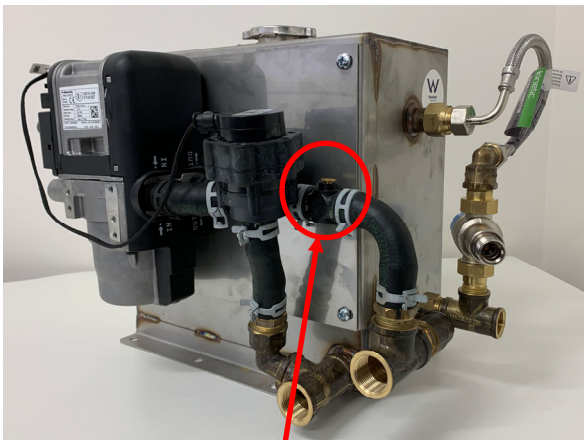
Fig. 24a Coolant line bleed valve
