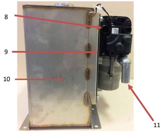
Fig 6 – Exhaust and Fuel Connection
