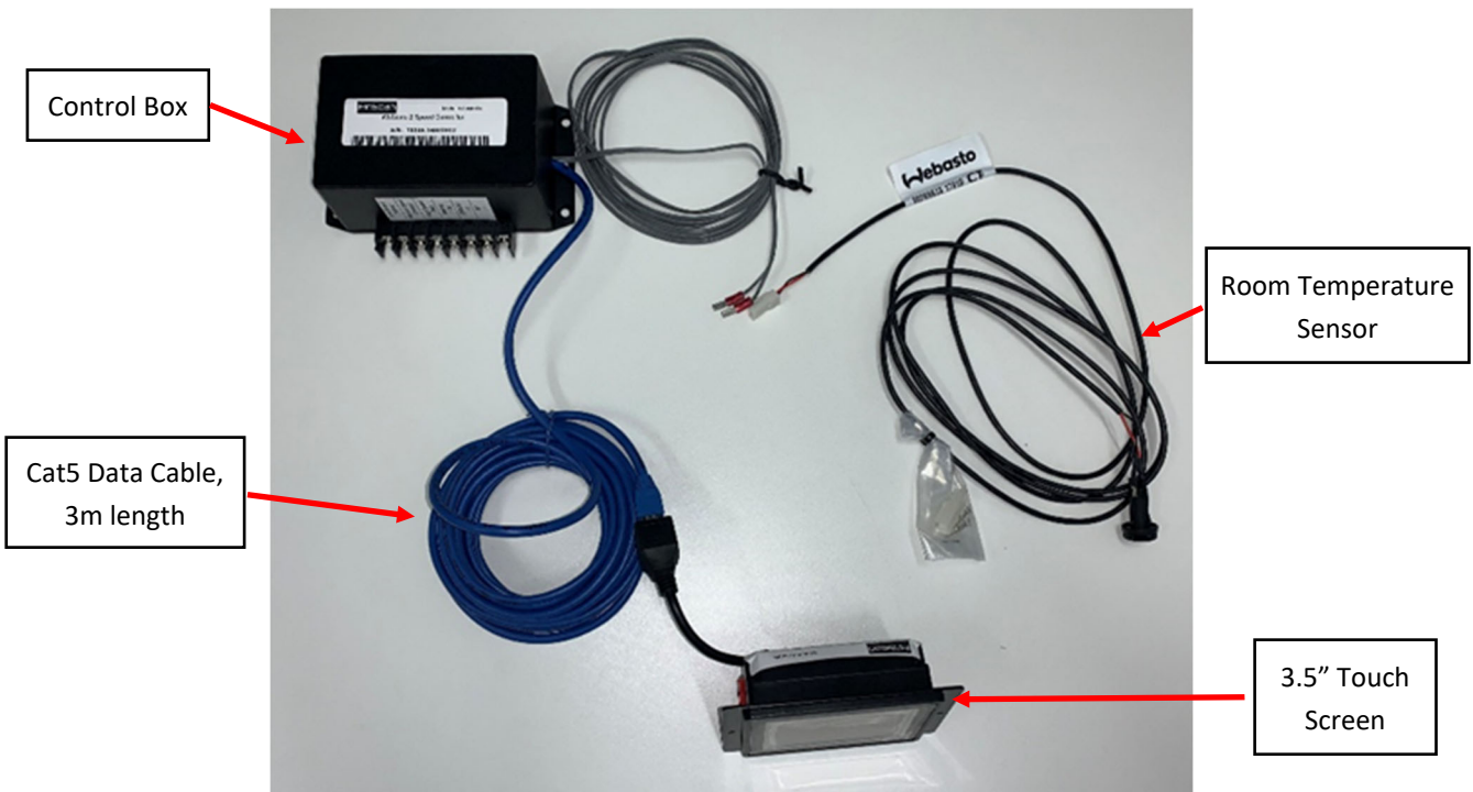
Fig. 27 Finscan control components
