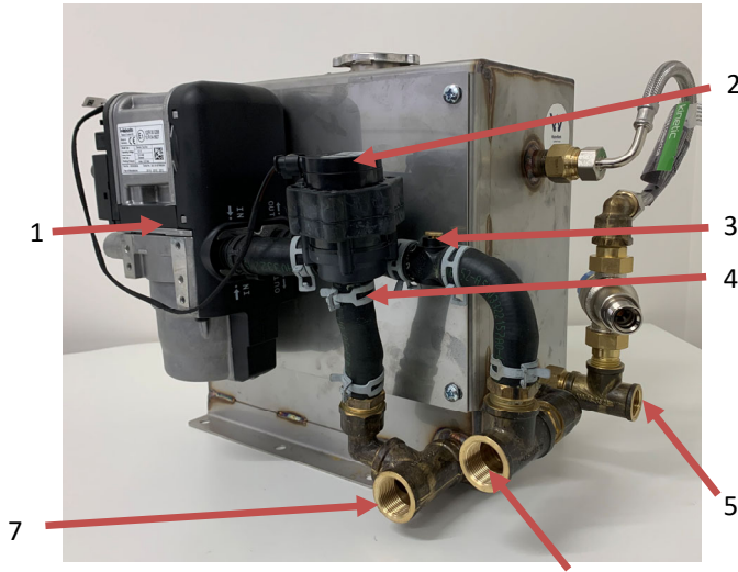
Fig 5 – Heater component location
