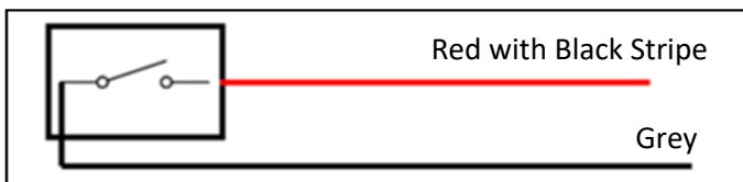
Fig 12 – On/Off Switch connection.
